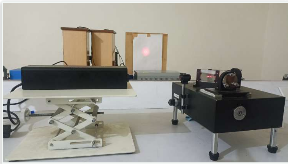
Michelson's Interferometer
