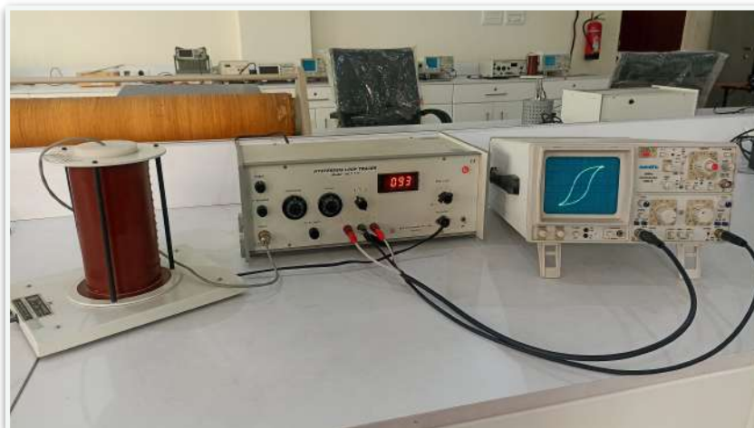
Hysteresis Loop Tracer
